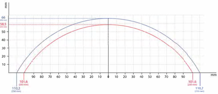
Castor Ø 235 / 250 mm
